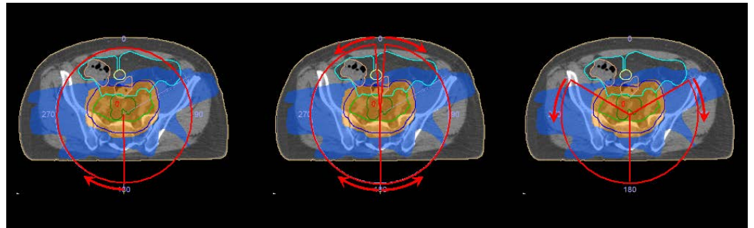
Figure 2. Potential arc arrangements for VMAT delivery. The single return arc arrangement (left) is sufficient for most patients but requires active optimisation to reduce the dose to anterior OARs. Split arc arrangement (centre) can be useful for complex cases. Partial arc arrangement (right) simplifies OAR sparing and is relatively robust to bowel OAR definition.
